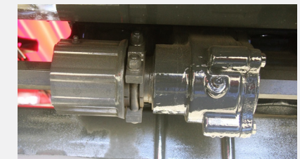
Each gathering set has an individual clutch. The auger has an individual clutch too.
